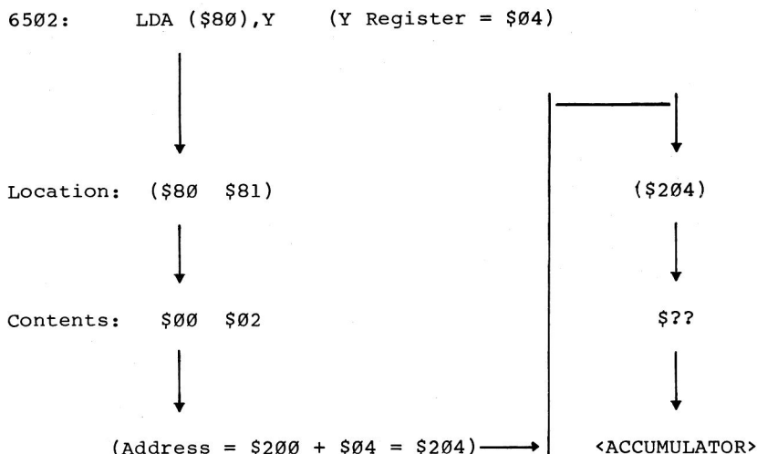
Figure 1. Indirect-indexed addressing.
